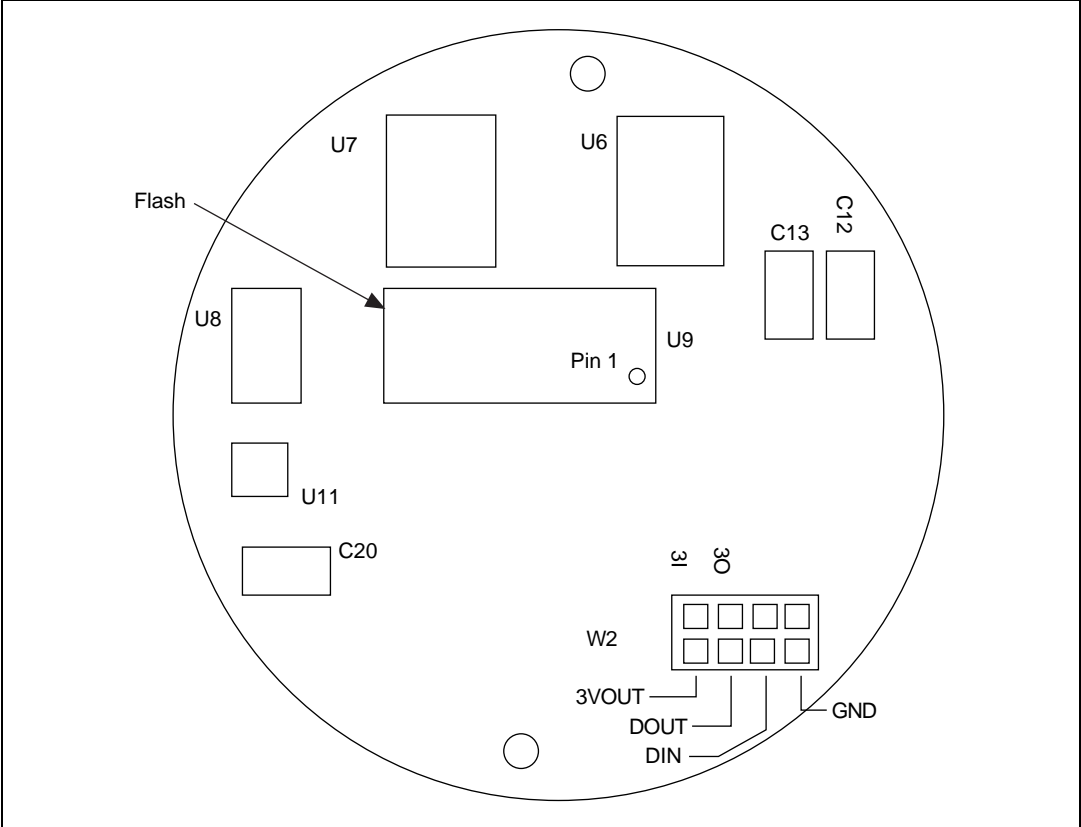
Figure 2-2. Bottom Side of 80188EB-Based Fieldbus Round Card
